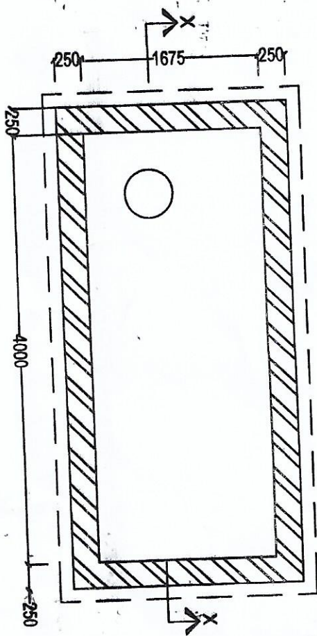
PLAN OF S.U.G. WATER RESERVOIR CAPACITY - 1000 GAL.S. SCALE - 1 : 50
